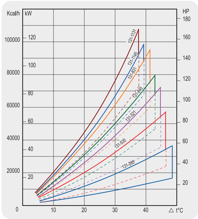
PERFORMANCE DIAGRAM At the maximum and minimum flow stated in schedule
